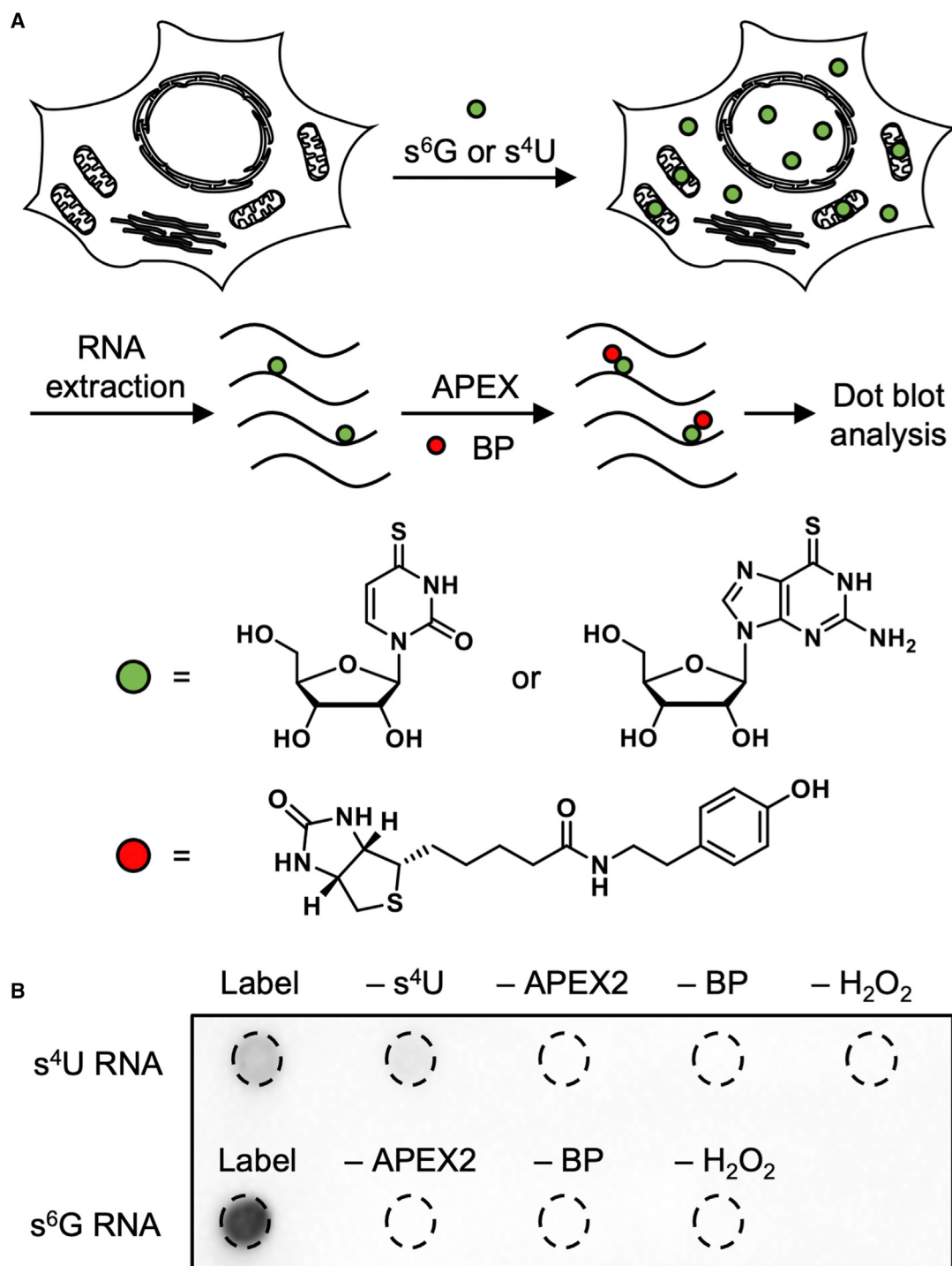
Figure 1. Development of APEX-mediated electron-rich ribonucleoside labeling strategy in vitro
